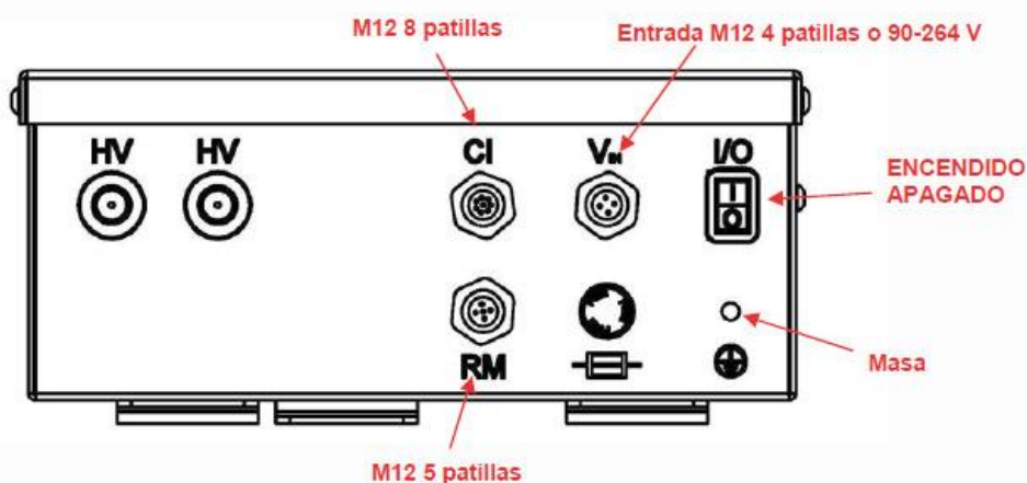
Panel frontal
